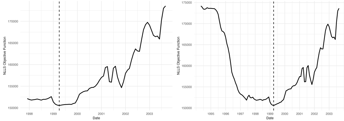
Figure 18: Change Point Detection in the AEM for Europe (Left: Both Trigger Points Changing, Right: Only Chromium Trigger Changing)
