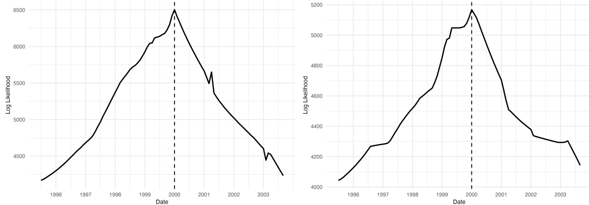
Figure 21: Change Point Detection in the CLEM for the US (Left: Both Trigger Points Changing, Right: Only Chromium Trigger Changing)
