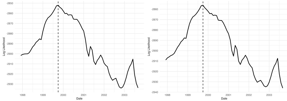
Figure 19: Change Point Detection in the CLEM for Europe (Left: Both Trigger Points Changing, Right: Only Chromium Trigger Changing)
