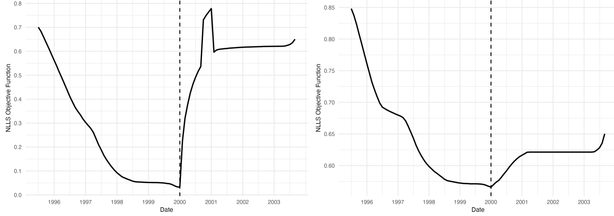
Figure 20: Change Point Detection in the AEM for the US (Left: Both Trigger Points Changing, Right: Only Chromium Trigger Changing)
